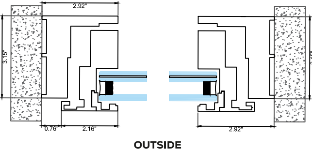
Horizontal Section
