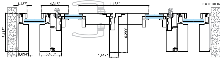
Horizontal section Option B
