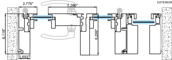
Horizontal section Option B
