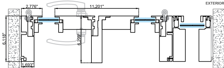
Horizontal section Option B
