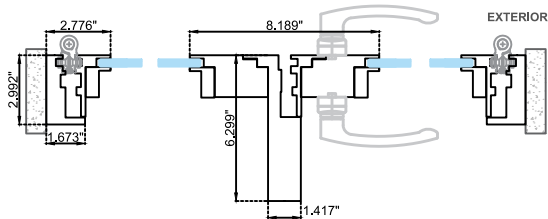
Horizontal section Option A
