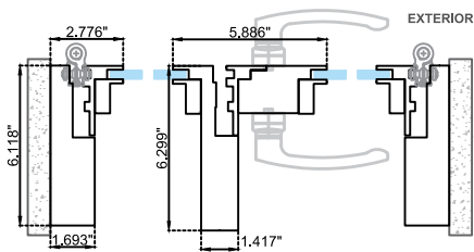
Horizontal section Option B
