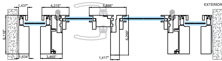
Horizontal section Option B
