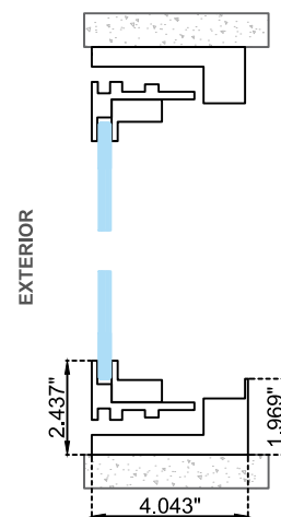
Vertical section Option A
