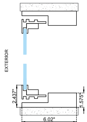
Vertical section Option B
