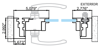
Horizontal section Option A
