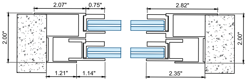
Horizontal Section
