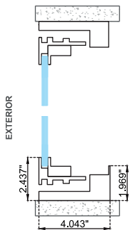
VERTICAL SECTION Option A
