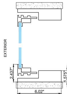
VERTICAL SECTION Option B
