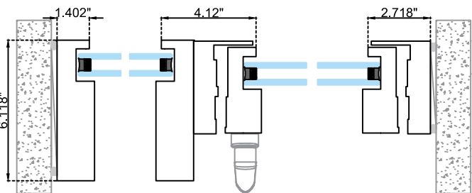
Horizontal Section
