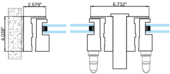
Double Sash
