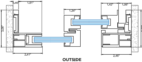
Horizontal Section
