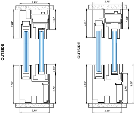
VERTICAL SECTION SILL COVER
