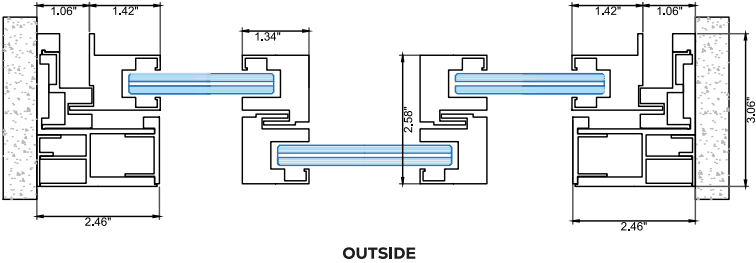
Horizontal Section
