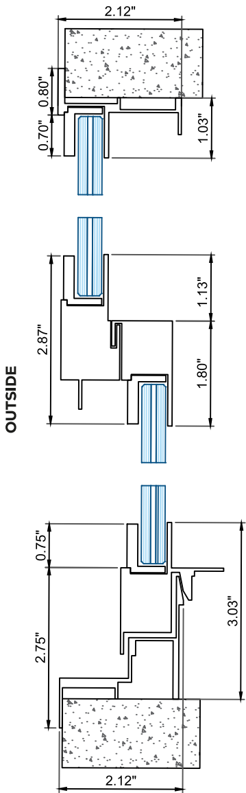
Vertical Section
