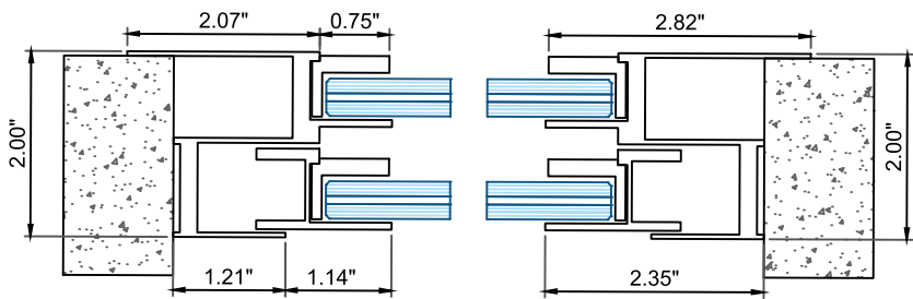
Horizontal Section
