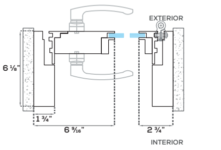
Option 2 Horizontal section
