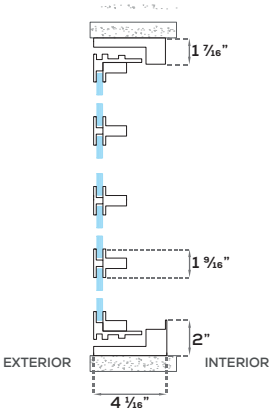
OPTION 1 VERTICAL SECTION Only available for Types: I – II
