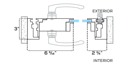
Option 1 Horizontal section
