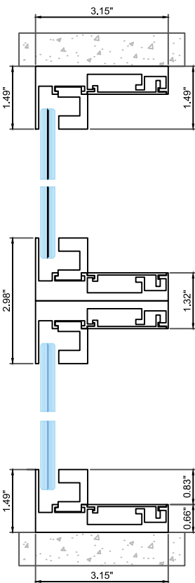
Vertical Section
