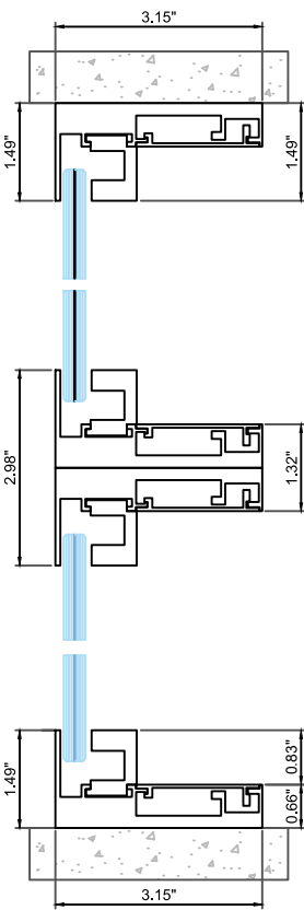
Vertical Section
