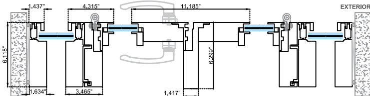
Horizontal section Option B
