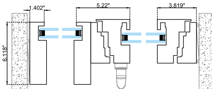
Single Sash + Fixed
