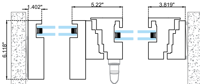
Horizontal Section
