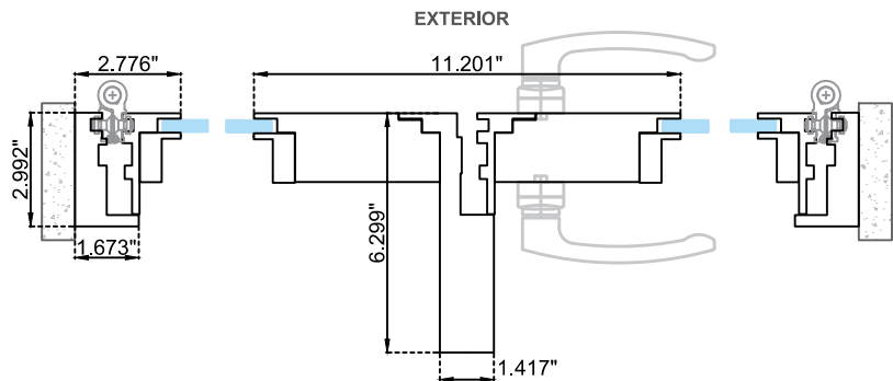
Horizontal section Option A
