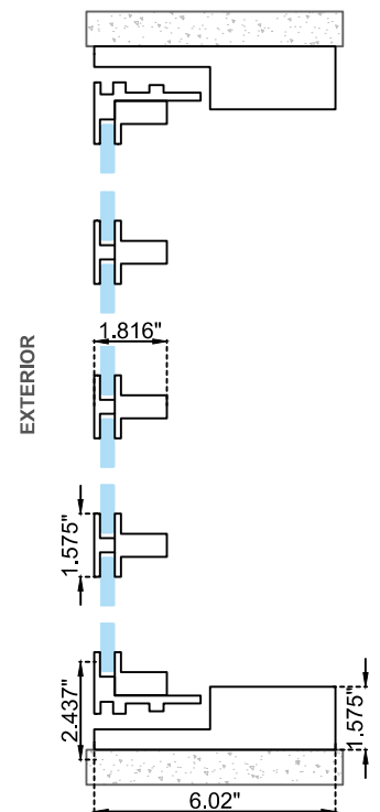
Vertical section Option B
