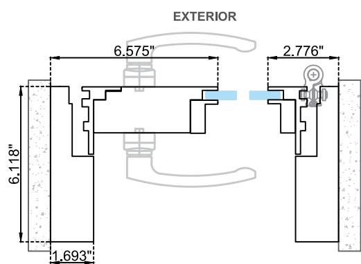
Horizontal section Option B
