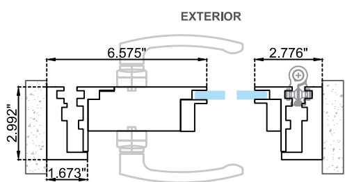
Horizontal section Option A
