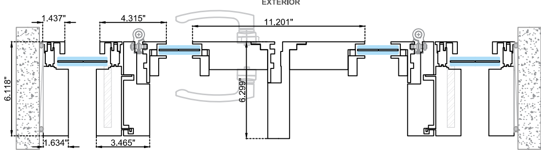
Horizontal section Option B
