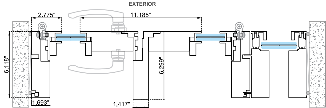
Horizontal section Option B
