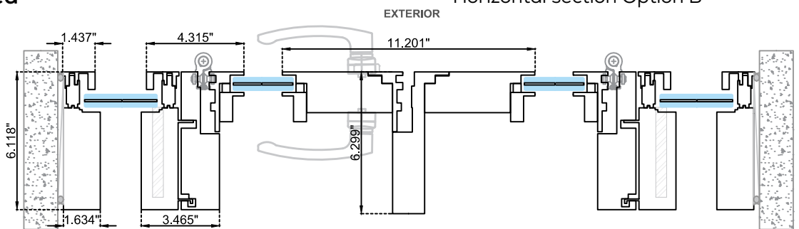
Horizontal section Option B
