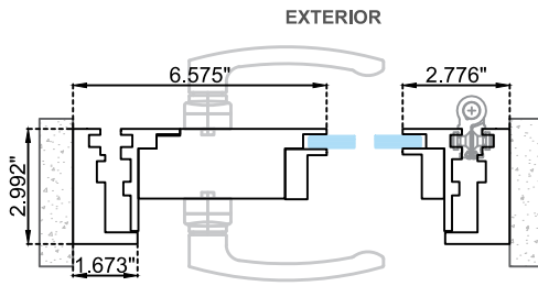
Horizontal section Option A
