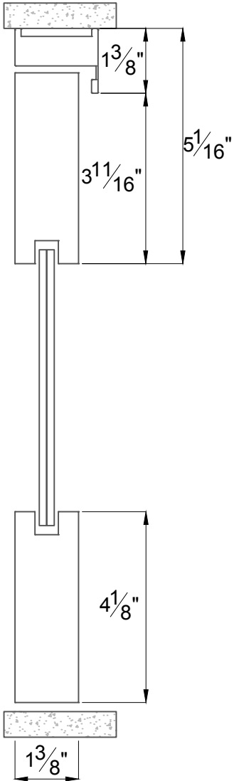
Section B-B'
