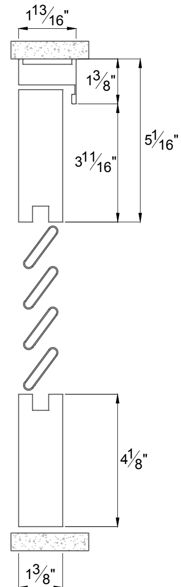
Section B-B'
