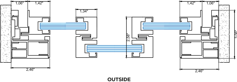
Horizontal Section
