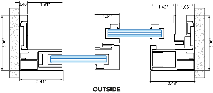
Horizontal Section
