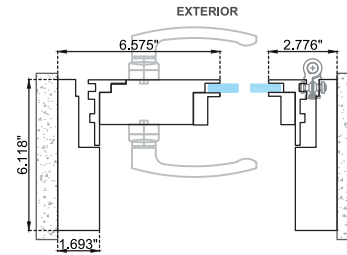
Horizontal section Option B
