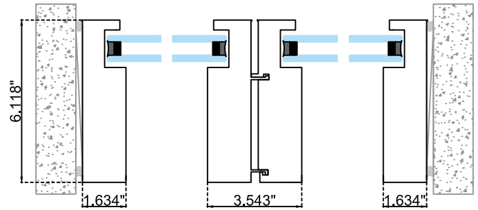
Horizontal Section
