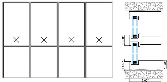
Horizontal Section
