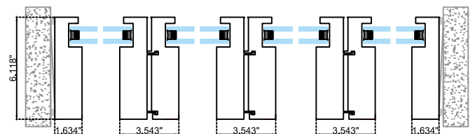
Horizontal Section
