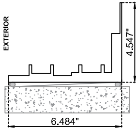
TRACK WITH SILL RISER
