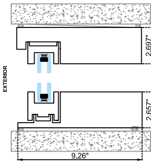
VERTICAL CROSS SECTION
