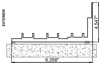
TRACK WITH SILL RISER
