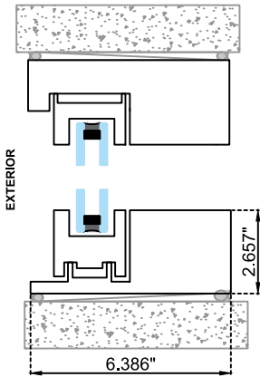
VERTICAL CROSS SECTION
