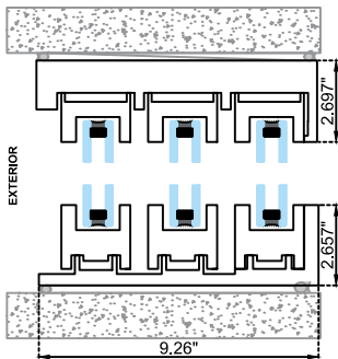
TRACK WITH SILL RISER
