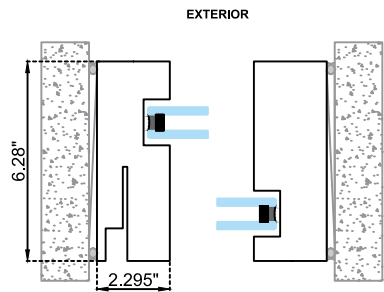
HORIZONTAL CROSS SECTION
