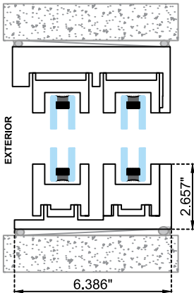
VERTICAL CROSS SECTION
