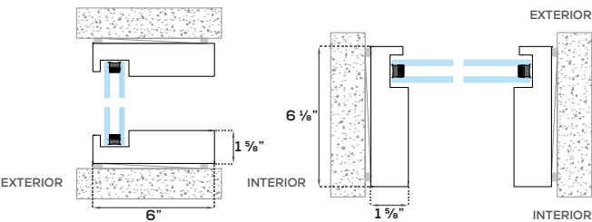
Single Fixed Panel
