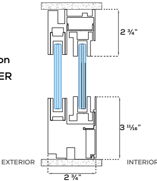
Horizontal Section
