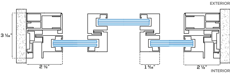
Horizontal Section
