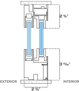
Vertical Section without SILL RISER
