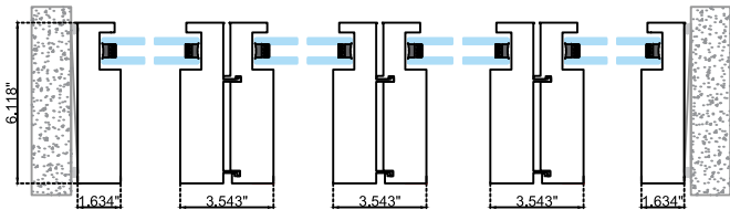
Horizontal Section
