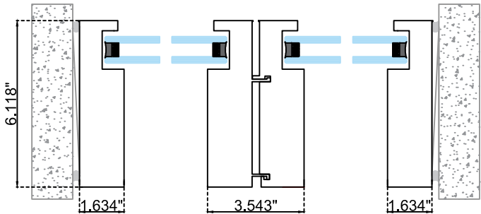
Horizontal Section
