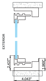
VERTICAL SECTION Option A
