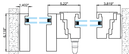
D. Single Sash+ Fixed
