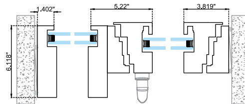
C. Single Sash + Fixed
