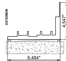
TRACK WITH SILL RISER
