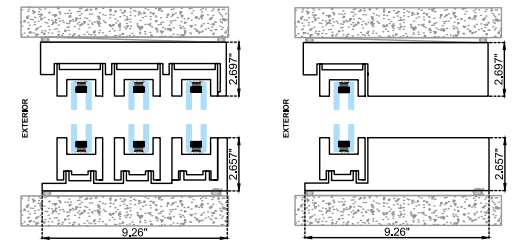
VERTICAL CROSS SECTION
