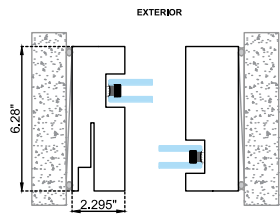
HORIZONTAL CROSS SECTION
