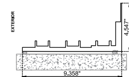
TRACK WITH SILL RISER
