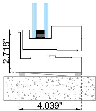
Full Frame
