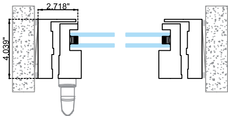
Single Sash
