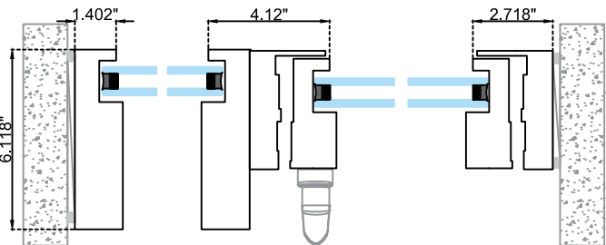
Horizontal Section
