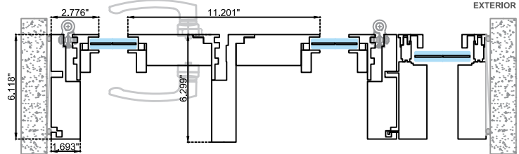
Horizontal section Option B
