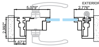
Horizontal section Option A
