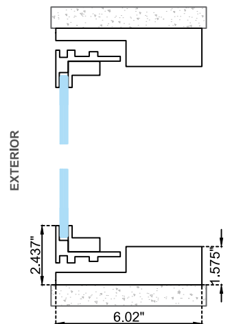
Vertical section Option B
