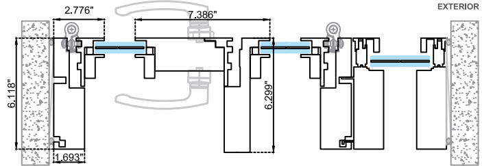
Horizontal section Option B
