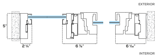
Single Sash + Fixed
