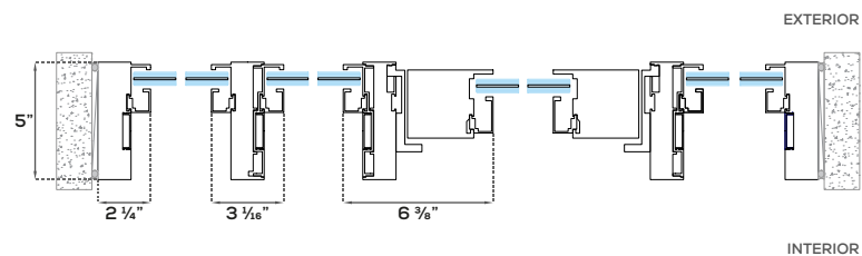
Single Door + Fixed Panel With Transom
