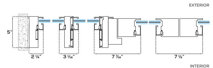
Double Door + Fixed Panel
