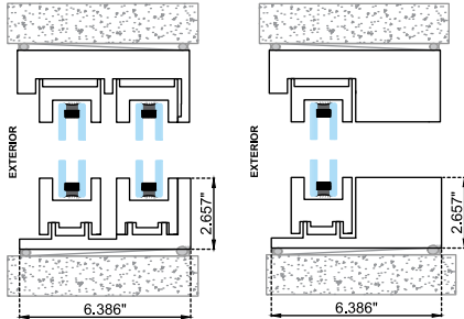
VERTICAL CROSS SECTION
