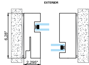
HORIZONTAL CROSS SECTION
