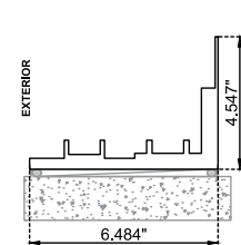
TRACK WITH SILL RISER
