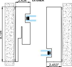
HORIZONTAL CROSS SECTION
