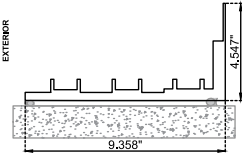
TRACK WITH SILL RISER
