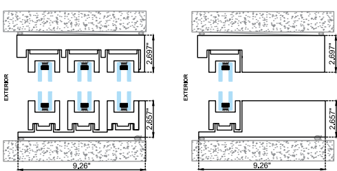
VERTICAL CROSS SECTION
